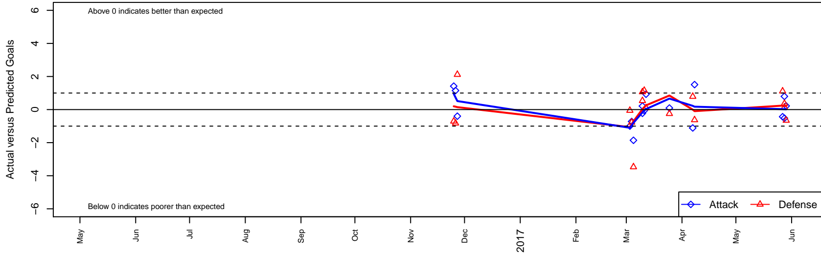
Las Vegas Sports Academy Red B00 Dots are actual minus expected GF (blue circles) and GA (red triangles). Blue line is smoothed change in attack strength. Red is smoothed change in defense strength.
